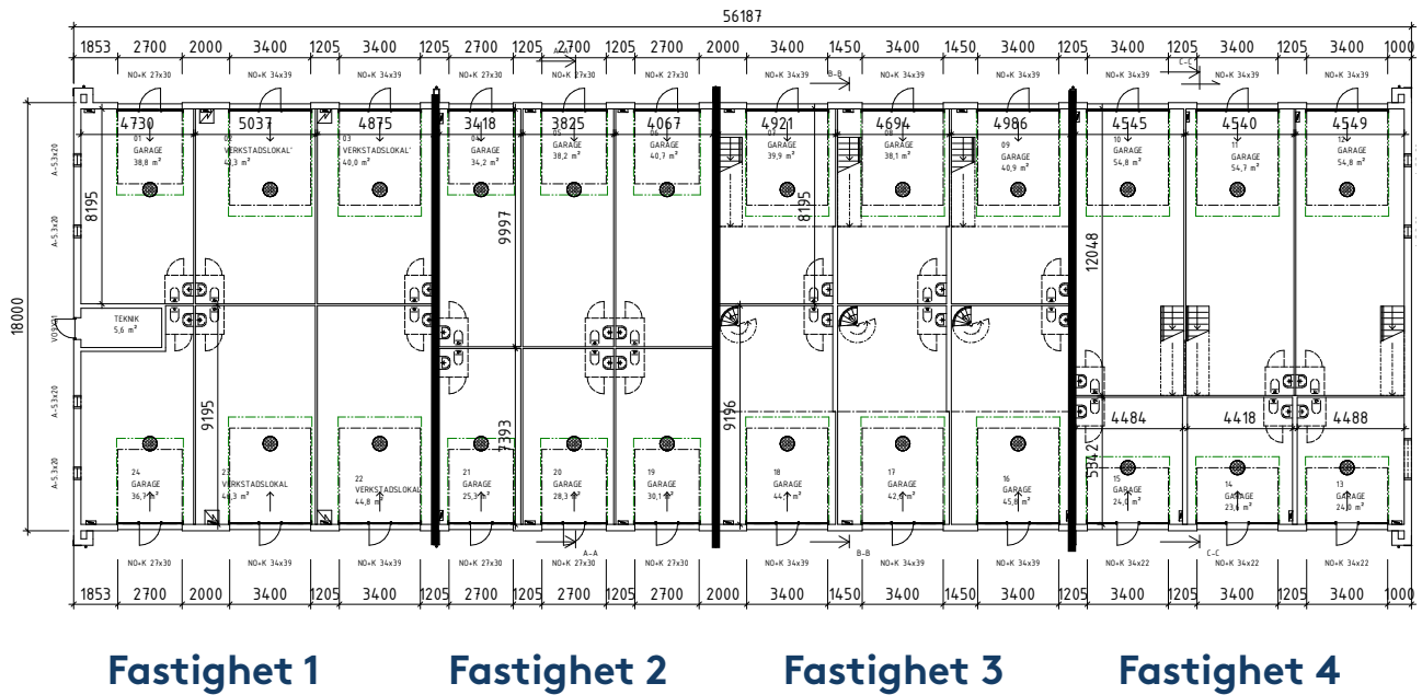
Plan 1
